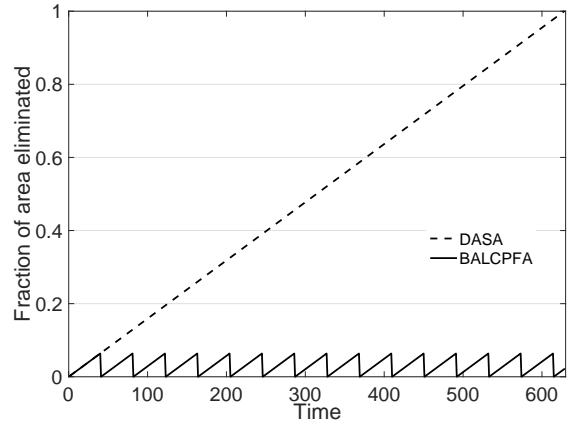
Figure 1: Plot of the fraction of area eliminated by a single agent ( R_v = 1, R = 20 ) vs. search time while foraging the arena using DASA and BALCPFA.
